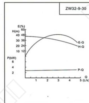
性能曲线 Performance Curve
